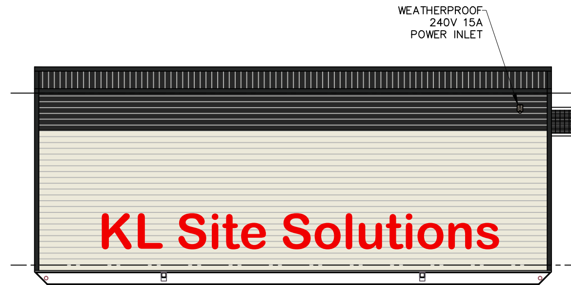
ELEVATION C.
